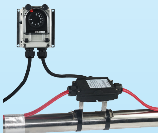
Example of assembly on two heat tracing cables, with Y26 connection box with stainless steel elevated bracket, for pipe antifreeze protection.
